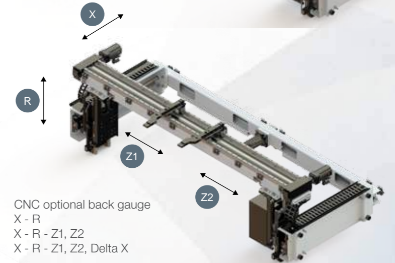
CNC back gauge X - R Z manuel X
